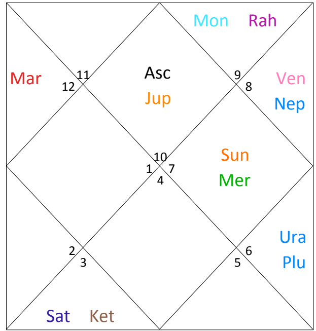
Co_Ordinates Of Planets
